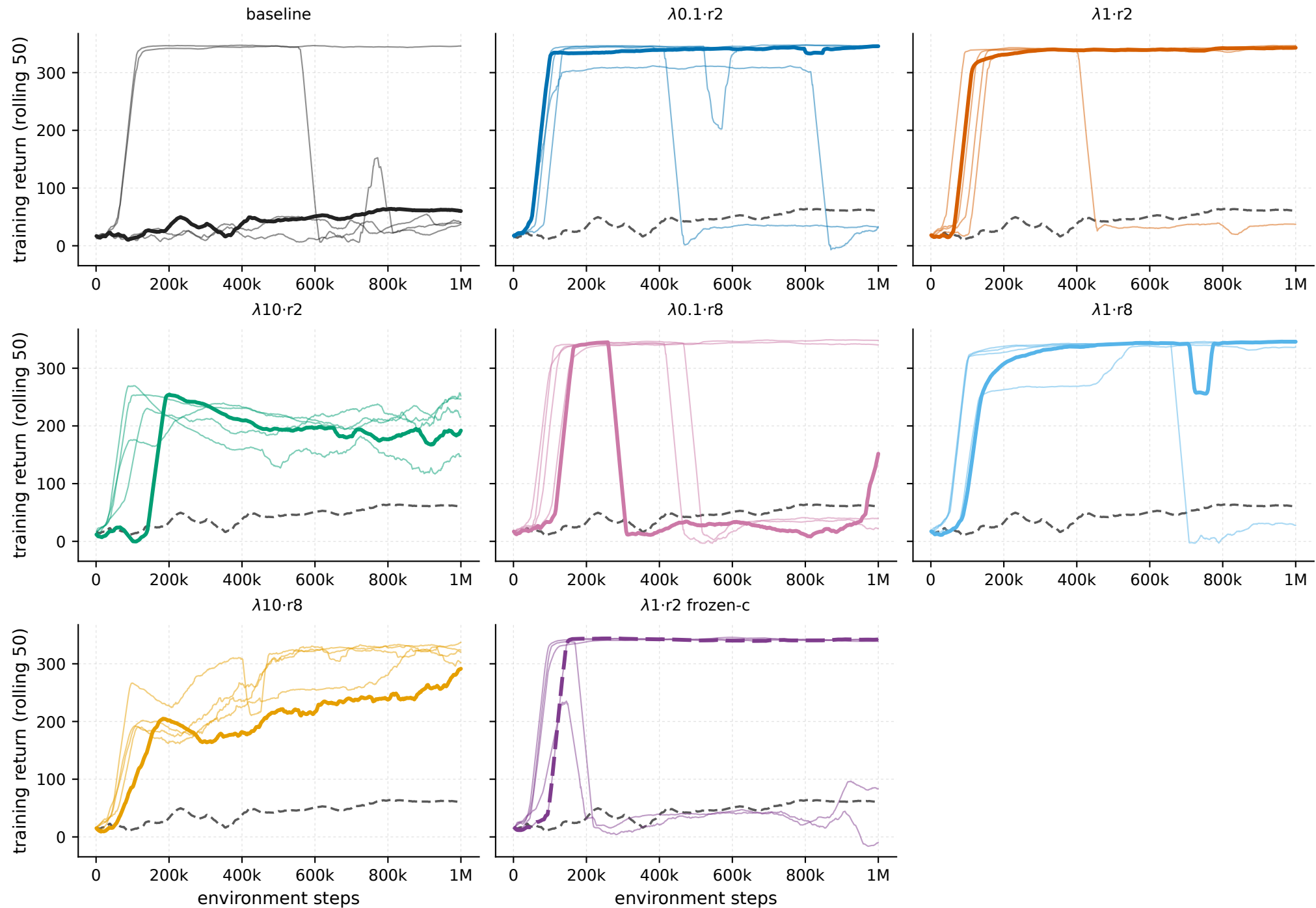
Swimmer-v5 - every seed per arm (train); grey dashed = baseline seed mean
