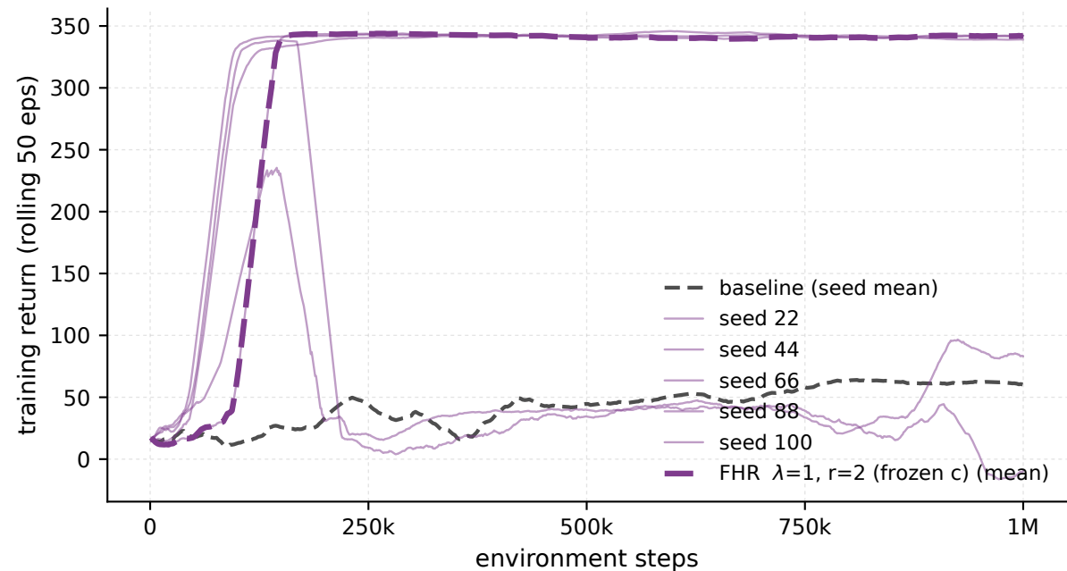
Swimmer-v5 - \lambda 1 \cdot r 2 frozen-c, every seed (train)
