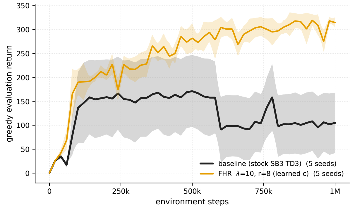
Swimmer-v5 - \lambda 10 \cdot r8 vs baseline (greedy eval)
