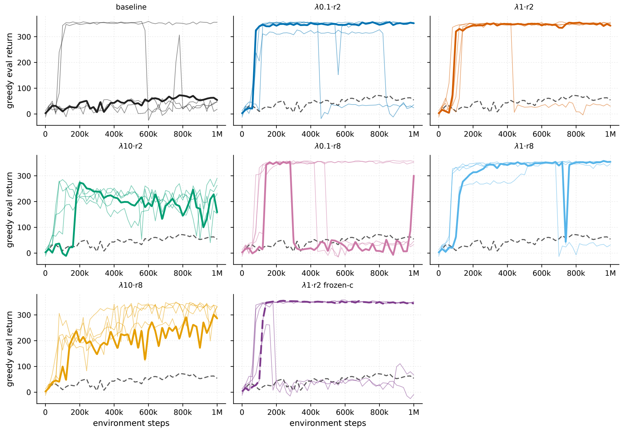
Swimmer-v5 - every seed per arm (eval); grey dashed = baseline seed mean
