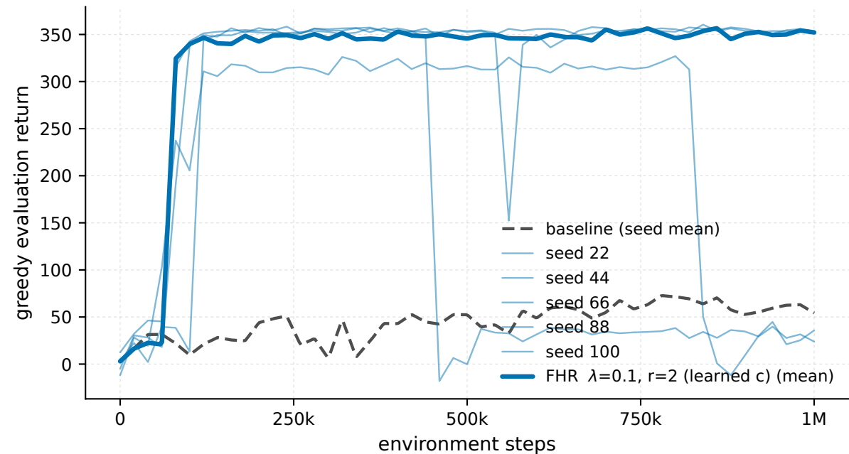
Swimmer-v5 - \lambda 0.1 \cdot r_2 , every seed (eval)
