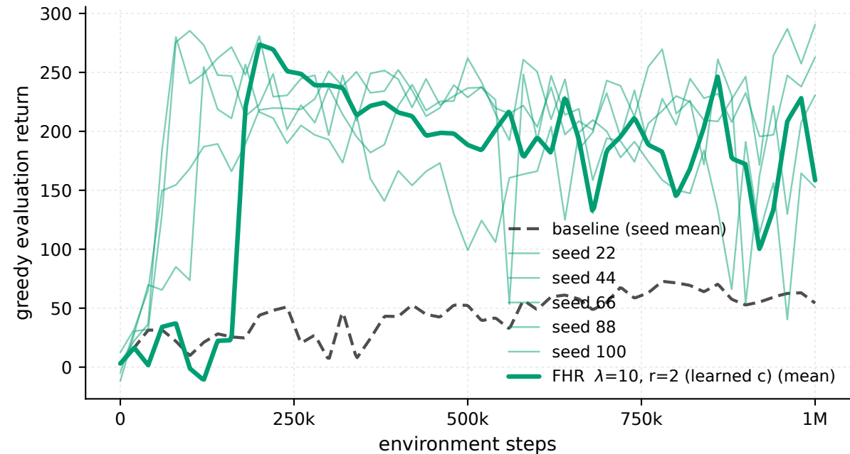
Swimmer-v5 - \lambda 10 \cdot r_2 , every seed (eval)
