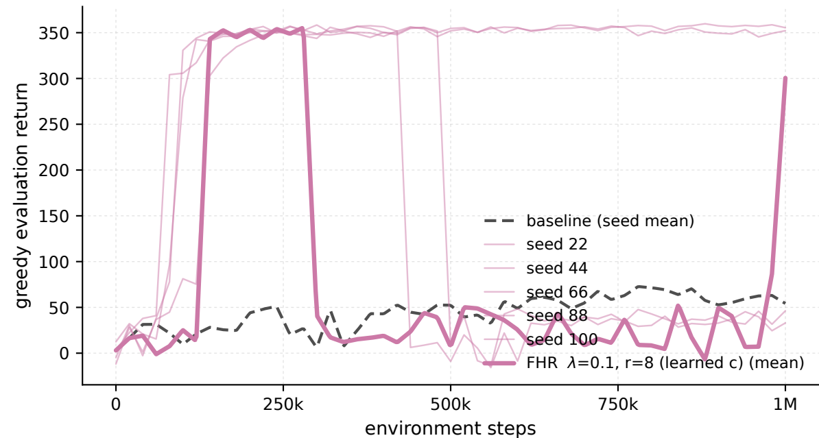
Swimmer-v5 - \lambda 0.1 \cdot r8 , every seed (eval)
