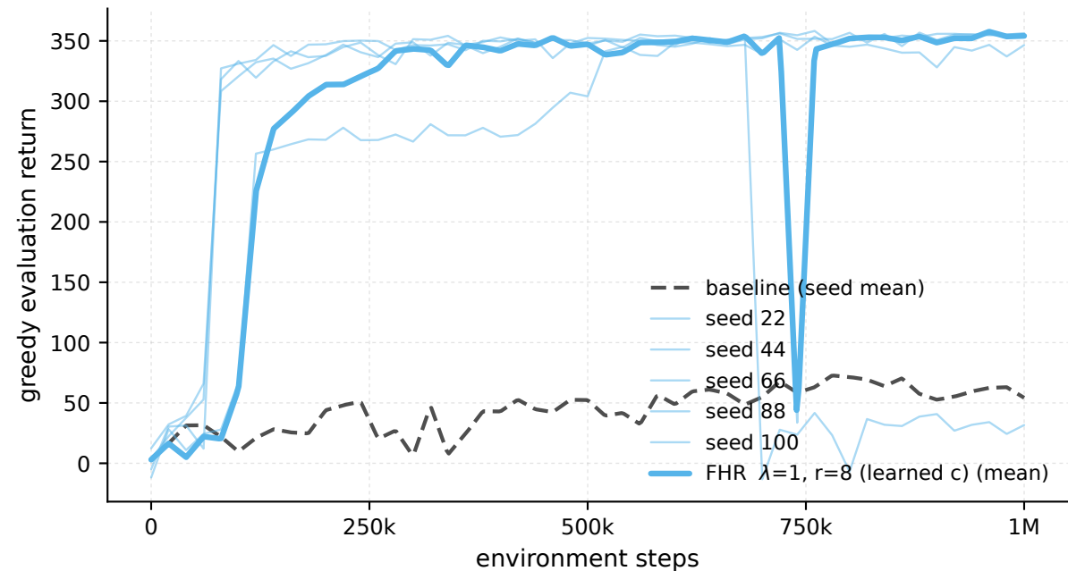
Swimmer-v5 - \lambda 1 \cdot r8 , every seed (eval)
