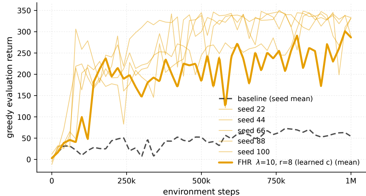
Swimmer-v5 - \lambda 10 \cdot r8 , every seed (eval)
