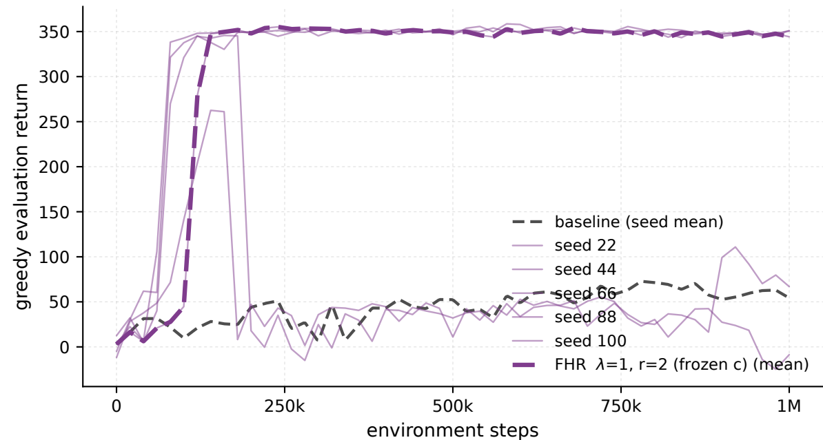
Swimmer-v5 - \lambda 1 \cdot r 2 frozen-c, every seed (eval)
