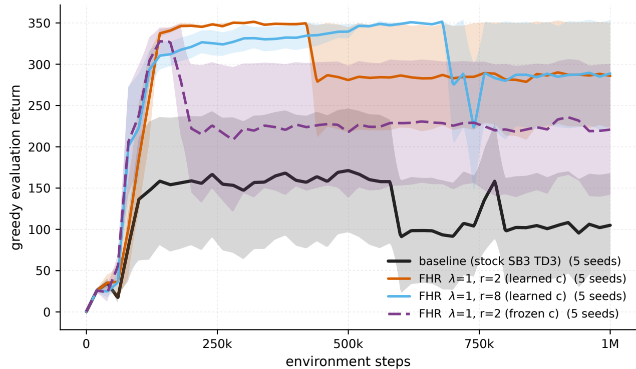
Swimmer-v5 - lambda = 1: learned vs frozen-theory c (eval)
