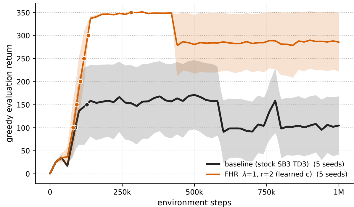
Swimmer-v5 - \lambda 1 \cdot r_2 vs baseline (greedy eval)
