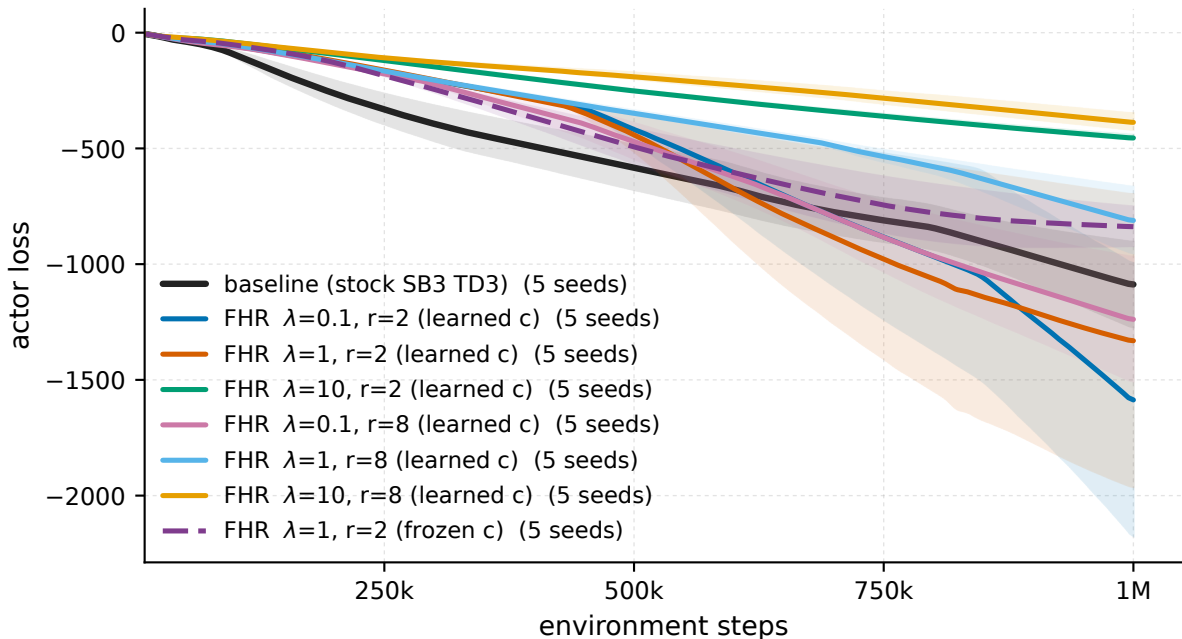
Swimmer-v5 - actor loss
