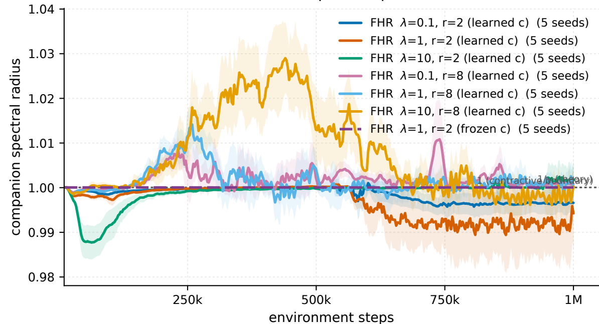
Swimmer-v5 - companion spectral radius
