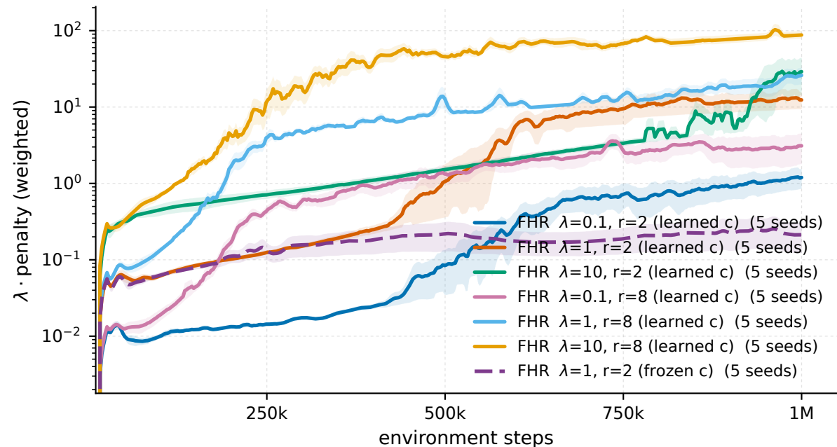
Swimmer-v5 - \lambda \cdot \text{penalty} (weighted)
