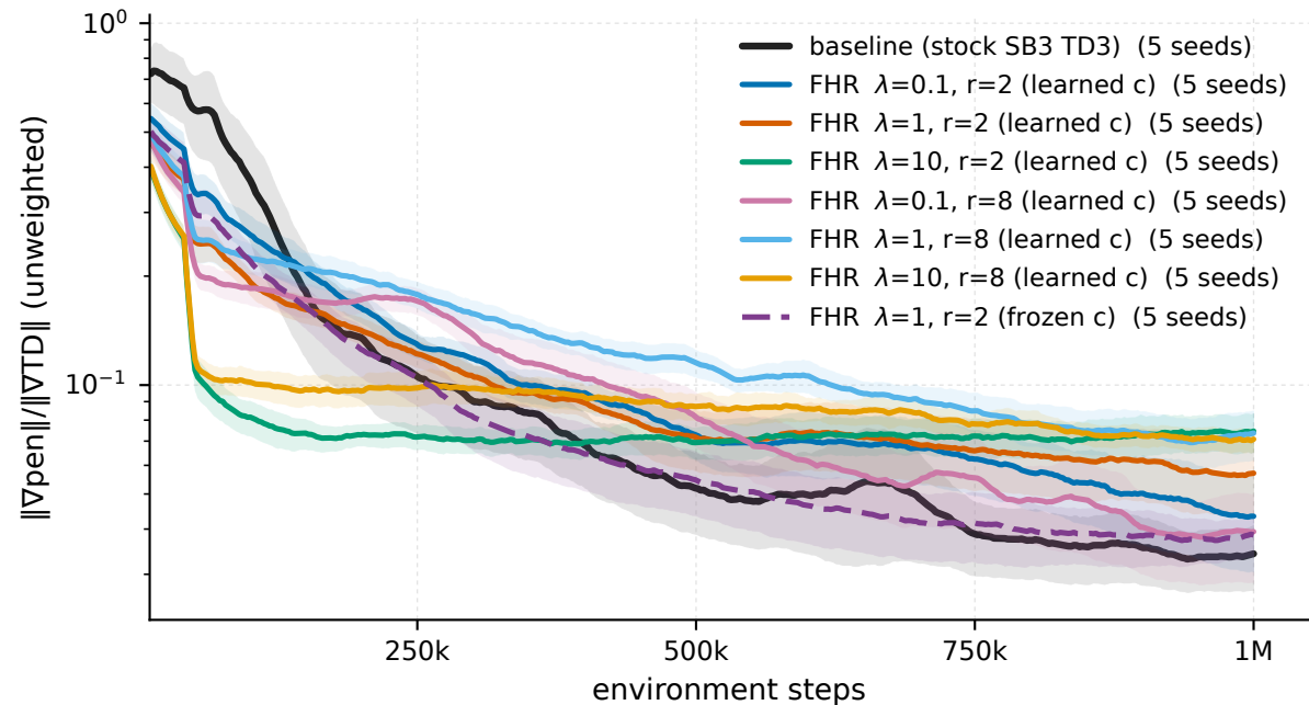
Swimmer-v5 - \|\nabla_{\text{pen}}\|/\|\nabla_{\text{TD}}\| (unweighted)
