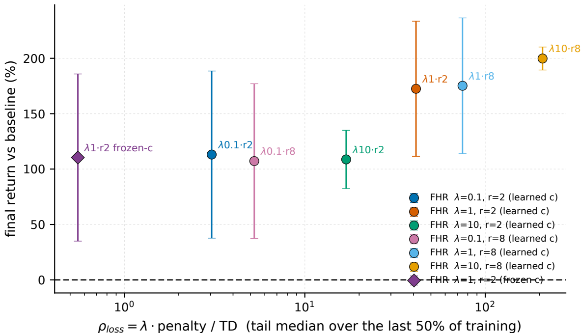
Swimmer-v5 - how hard the penalty pushes vs what it buys
