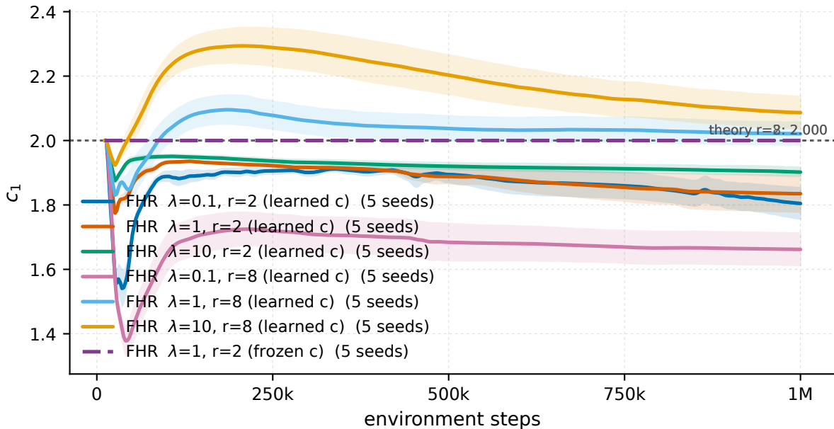
Swimmer-v5 - recurrence coefficient c_1 vs the Bellman theory value
