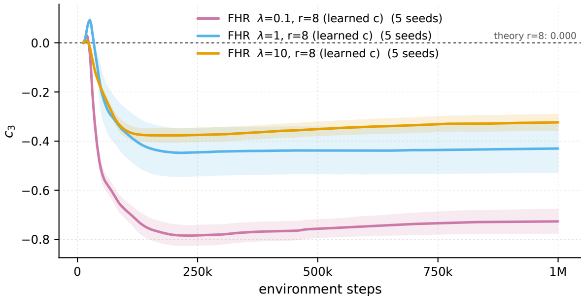
Swimmer-v5 - recurrence coefficient c_3 vs the Bellman theory value
