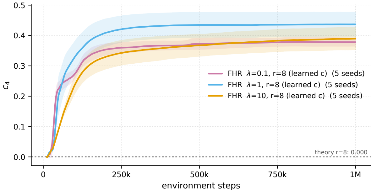
Swimmer-v5 - recurrence coefficient c_4 vs the Bellman theory value
