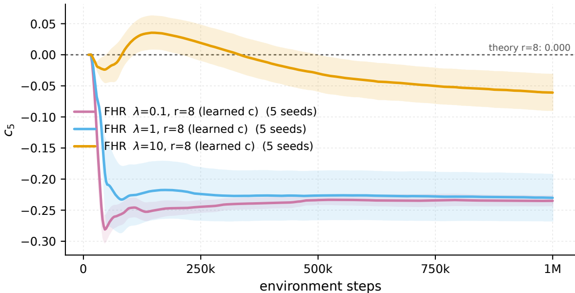
Swimmer-v5 - recurrence coefficient c_5 vs the Bellman theory value
