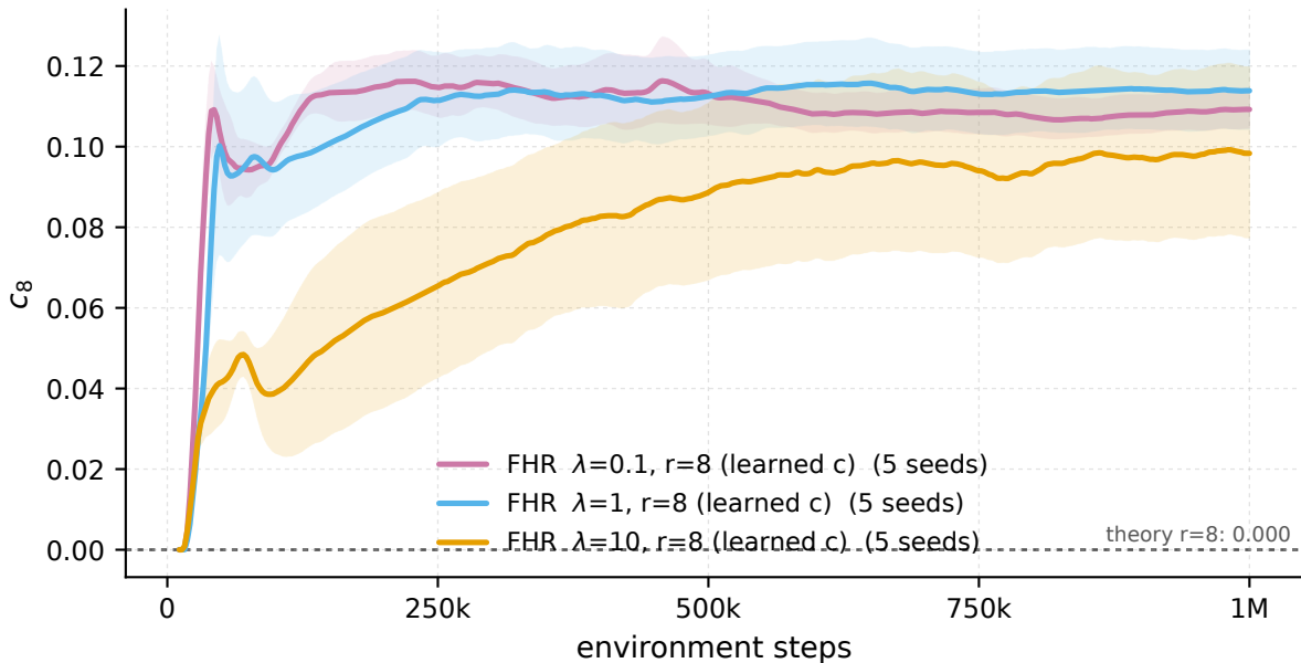
Swimmer-v5 - recurrence coefficient c_8 vs the Bellman theory value
