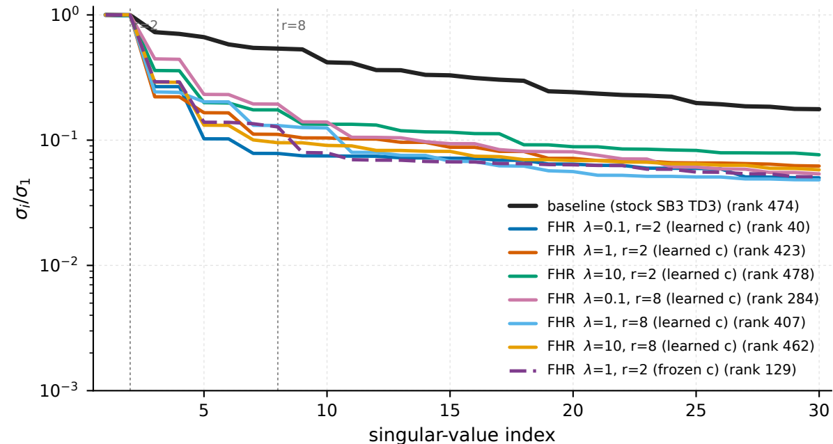
Swimmer-v5 - Hankel( \pi(s_t)_0 ) of the final policy (action dim 0)
