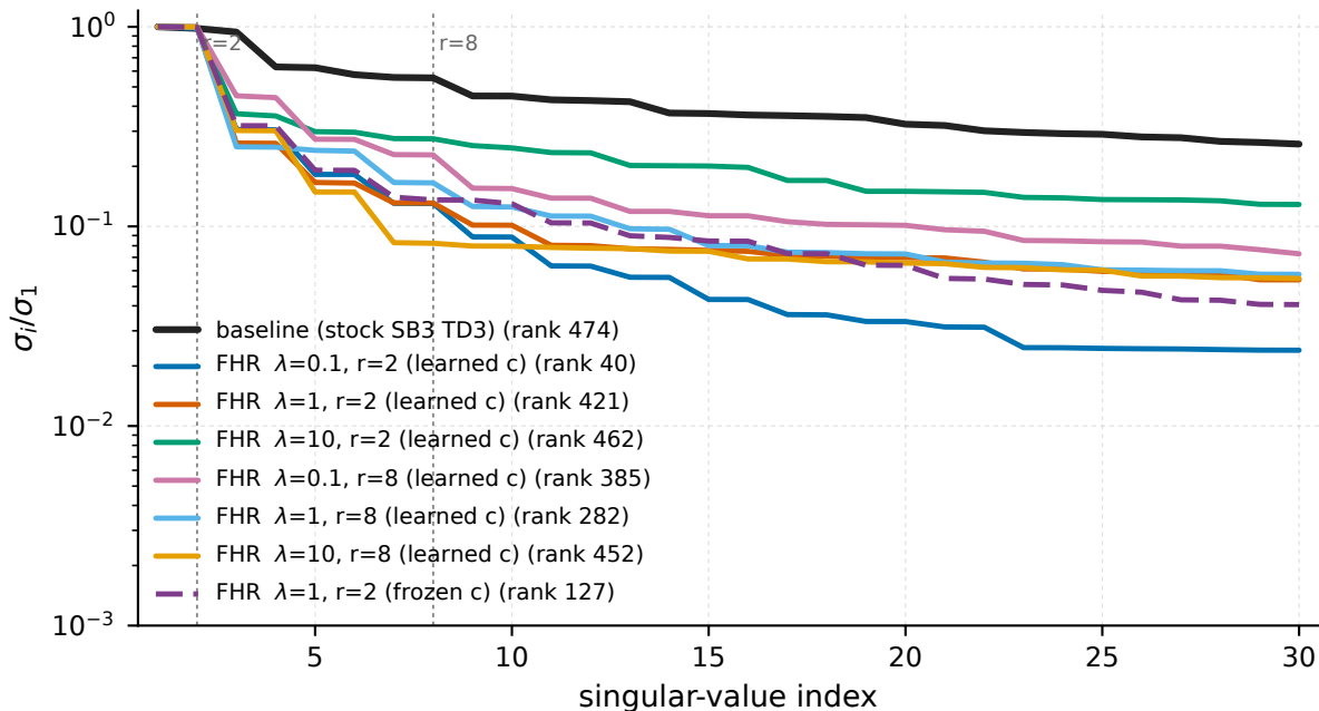
Swimmer-v5 - Hankel( \pi(s_t)_1 ) of the final policy (action dim 1)
