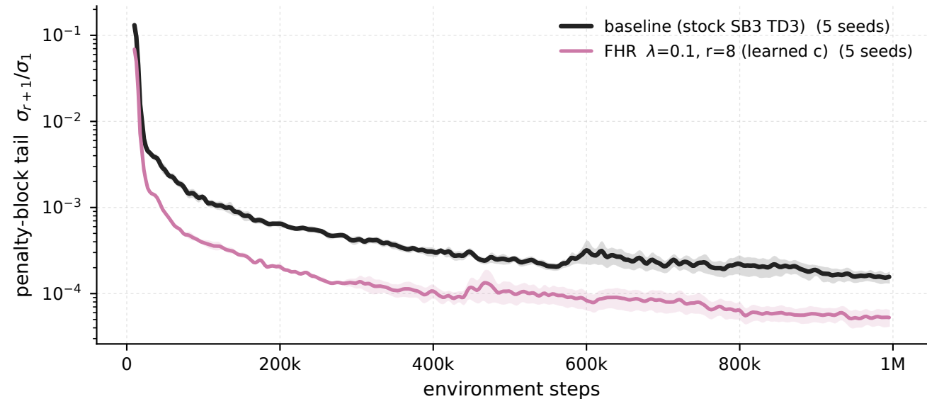
Swimmer-v5 - \lambda 0.1 \cdot r8 vs baseline, penalised windows penalty-block tail \sigma_{r+1}/\sigma_1
