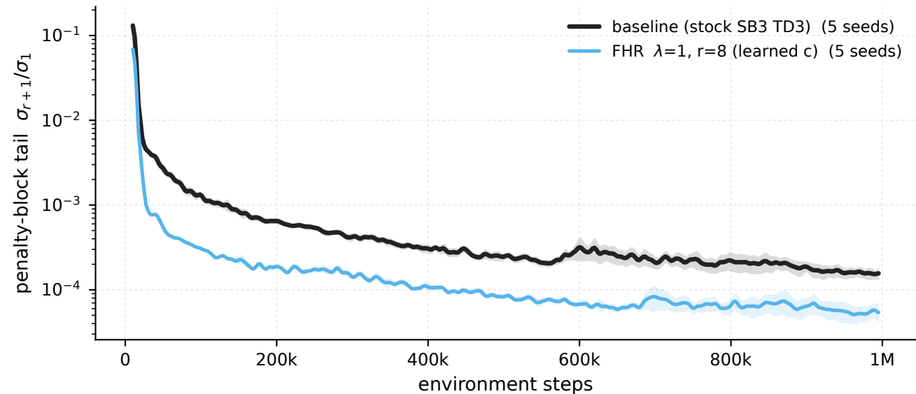
Swimmer-v5 - \lambda 1 \cdot r8 vs baseline, penalised windows penalty-block tail \sigma_{r+1}/\sigma_1
