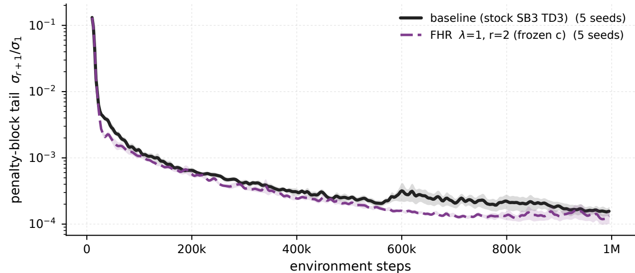
Swimmer-v5 - \lambda 1 \cdot r_2 frozen-c vs baseline, penalised windows penalty-block tail \sigma_{r+1}/\sigma_1
