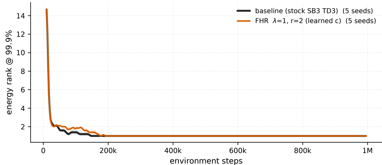
Swimmer-v5 - \lambda 1 \cdot r_2 vs baseline, penalised windows energy rank @ 99.9%
