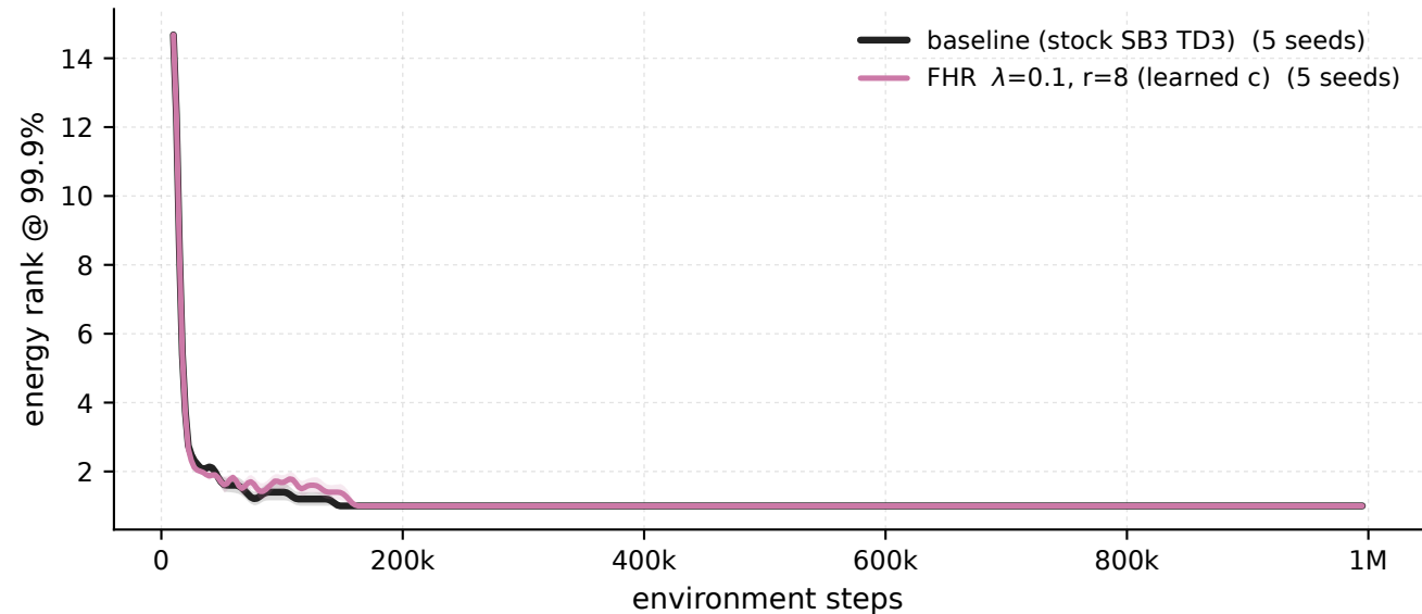
Swimmer-v5 - \lambda 0.1 \cdot r8 vs baseline, penalised windows energy rank @ 99.9%
