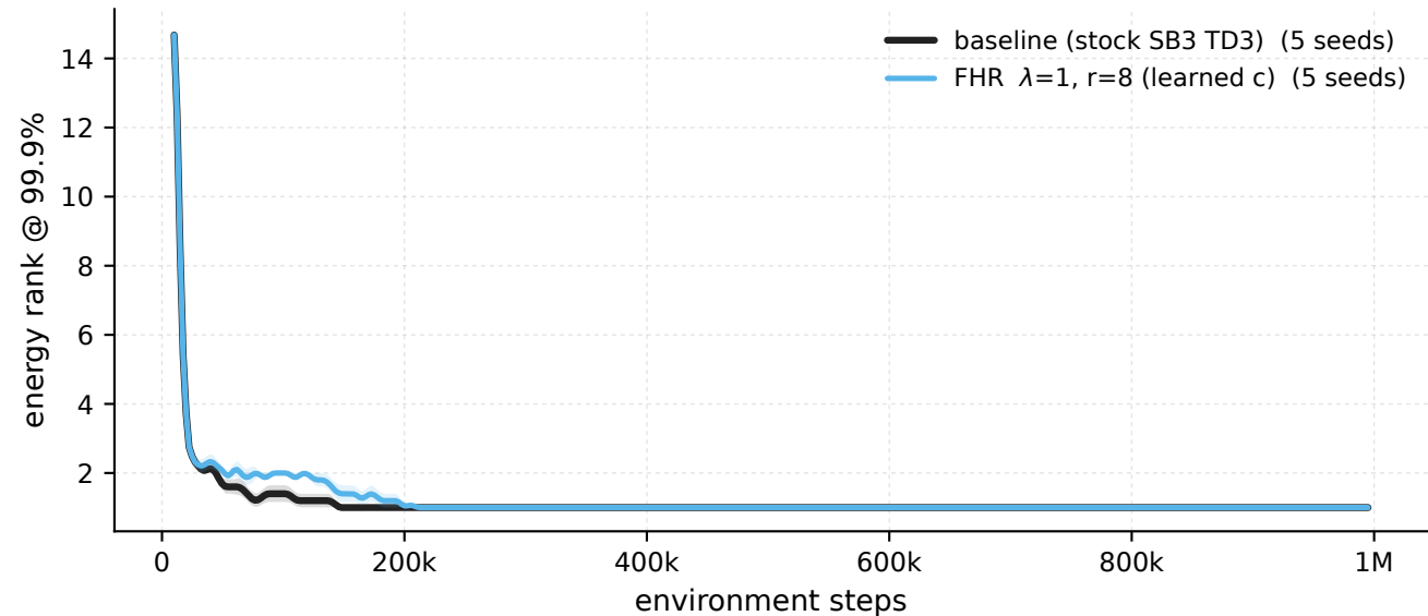
Swimmer-v5 - \lambda 1 \cdot r8 vs baseline, penalised windows energy rank @ 99.9%
