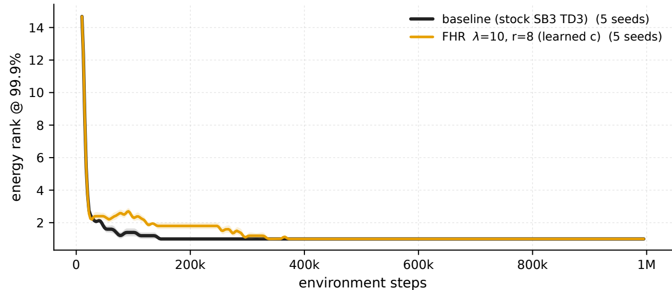
Swimmer-v5 - \lambda 10 \cdot r8 vs baseline, penalised windows energy rank @ 99.9%
