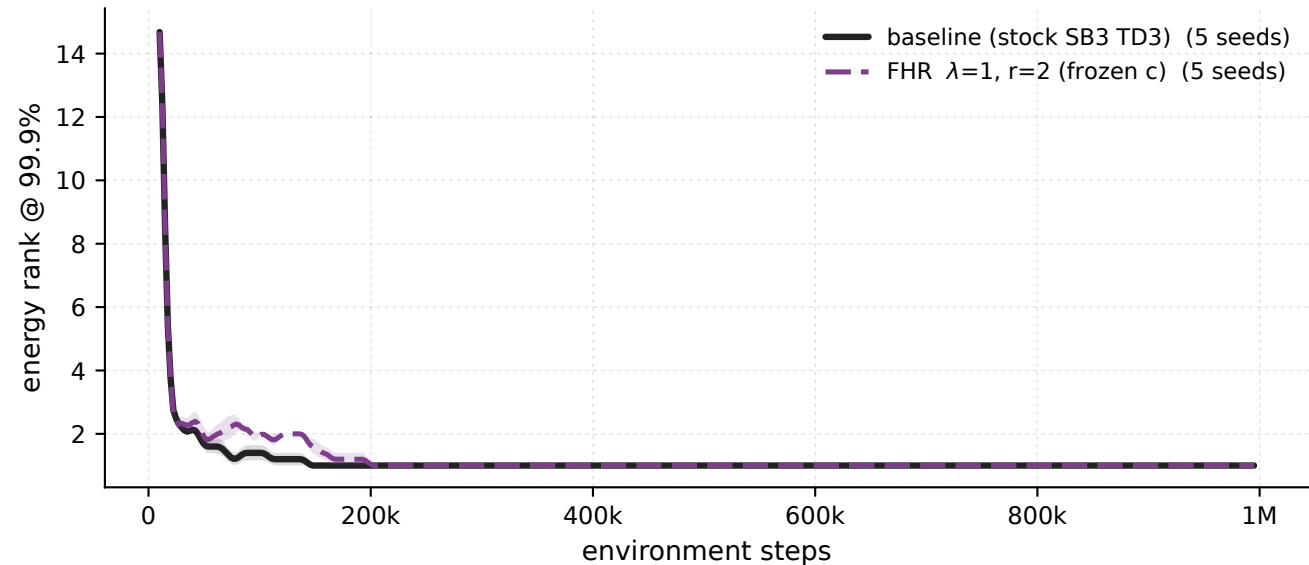
Swimmer-v5 - \lambda 1 \cdot r 2 frozen-c vs baseline, penalised windows energy rank @ 99.9%
