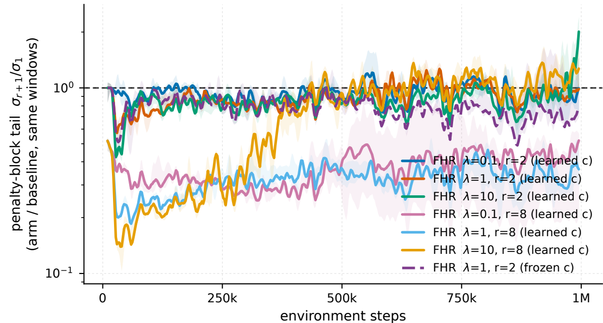
Swimmer-v5 - compression relative to the baseline
