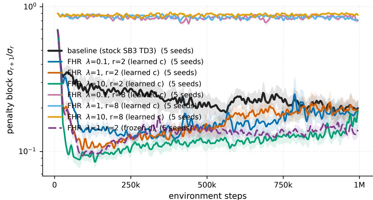
Swimmer-v5 - penalised windows: \sigma_{r+1}/\sigma_r of the penalty block
