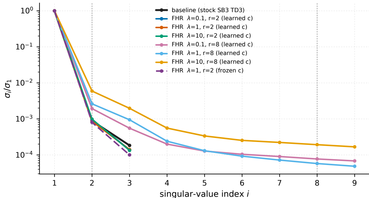
Swimmer-v5 - penalty block spectrum, final 25% of training (median over seeds and critics)
