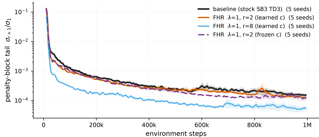
Swimmer-v5 - \lambda 1 \cdot r2 , \lambda 1 \cdot r8 , \lambda 1 \cdot r2 frozen-c vs baseline, penalised windows penalty-block tail \sigma_{r+1}/\sigma_1
