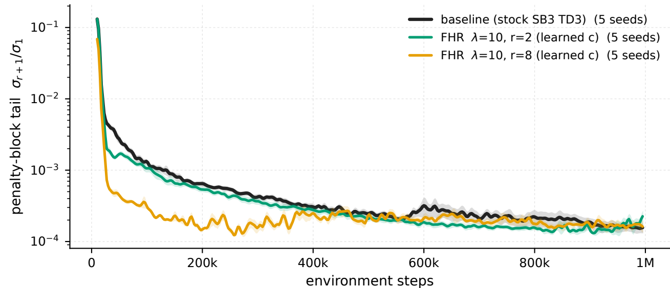
Swimmer-v5 - \lambda 10 \cdot r_2 , \lambda 10 \cdot r_8 vs baseline, penalised windows penalty-block tail \sigma_{r+1}/\sigma_1
