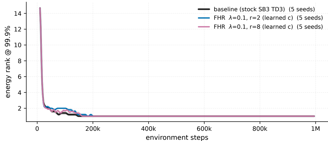
Swimmer-v5 - \lambda 0.1 \cdot r_2 , \lambda 0.1 \cdot r_8 vs baseline, penalised windows energy rank @ 99.9%
