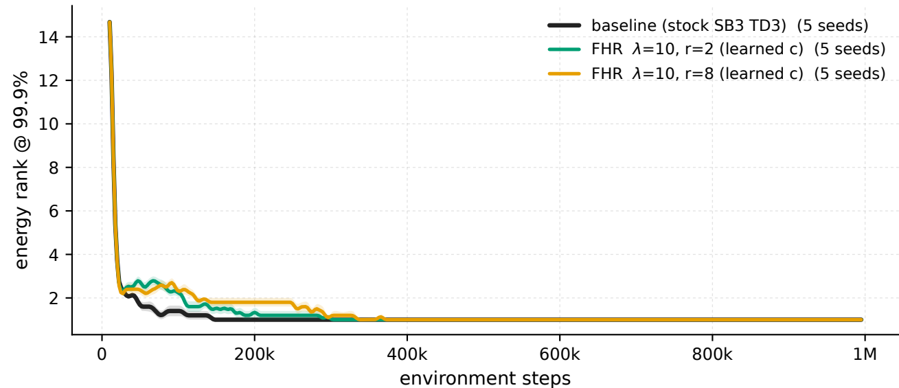
Swimmer-v5 - \lambda 10 \cdot r_2 , \lambda 10 \cdot r_8 vs baseline, penalised windows energy rank @ 99.9%
