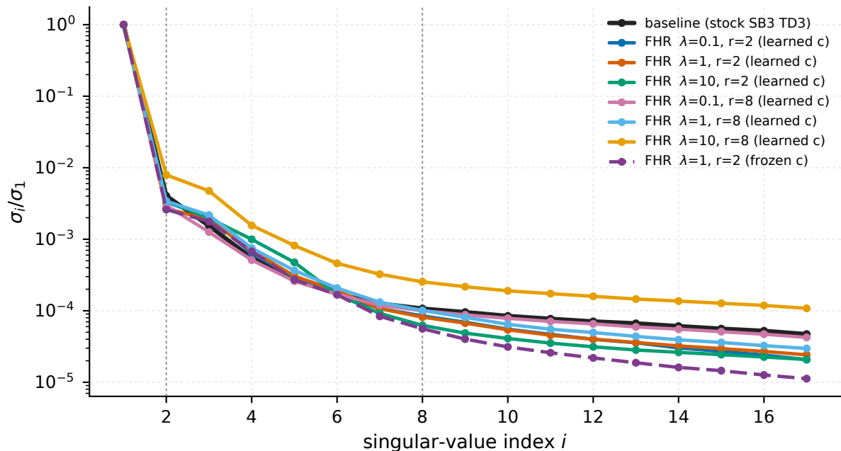
Swimmer-v5 - replay window spectrum, final 25% of training (median over seeds and critics)
