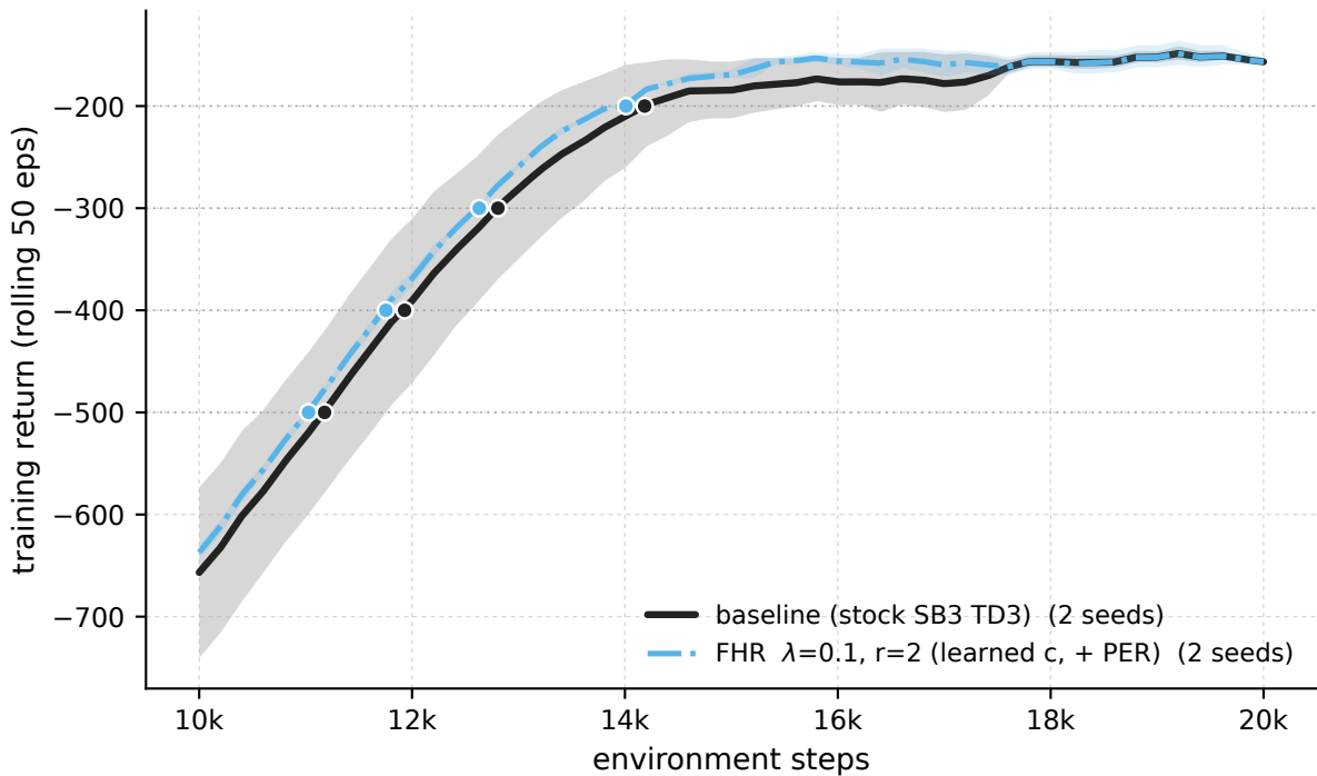
Pendulum-v1 - \lambda 0.1 \cdot r_2 +PER vs baseline (training stream)
