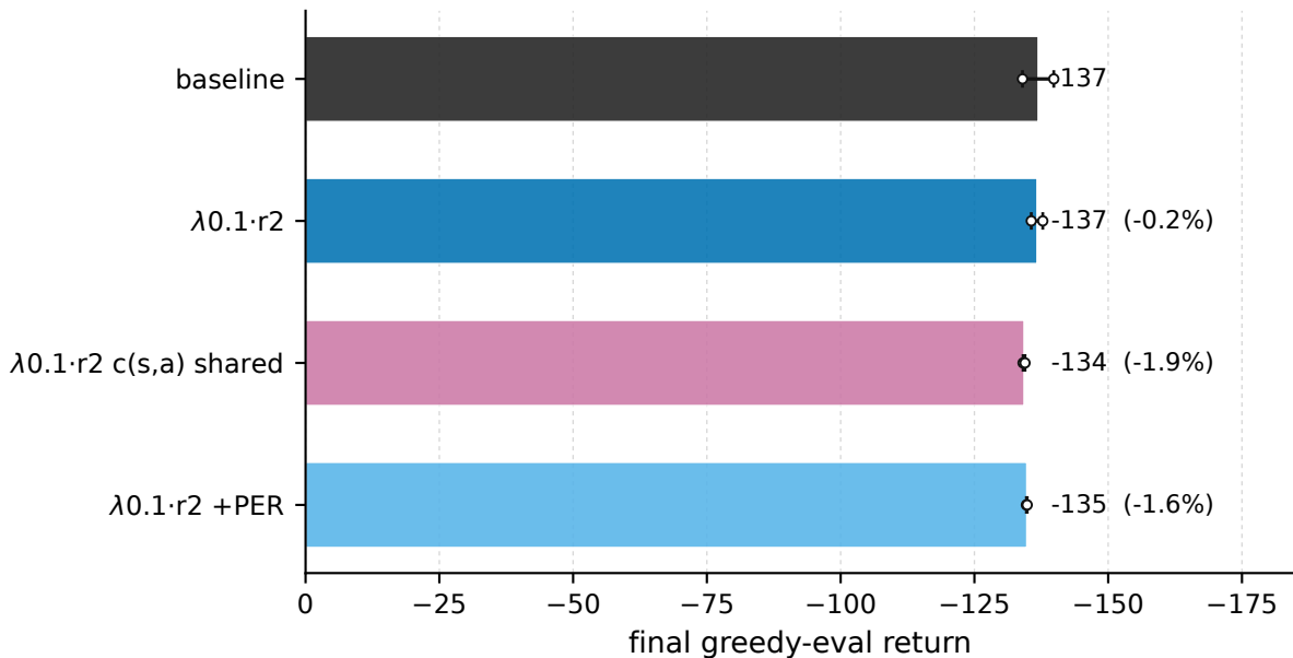
Pendulum-v1 - final return, \lambda = 0.1 vs baseline
