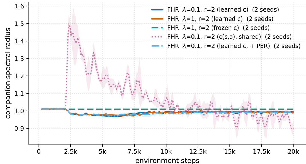
Pendulum-v1 - companion spectral radius
