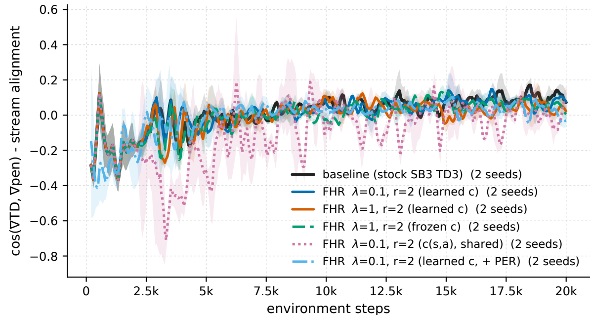
Pendulum-v1 - \cos(\nabla\text{TD}, \nabla\text{pen}) - stream alignment
