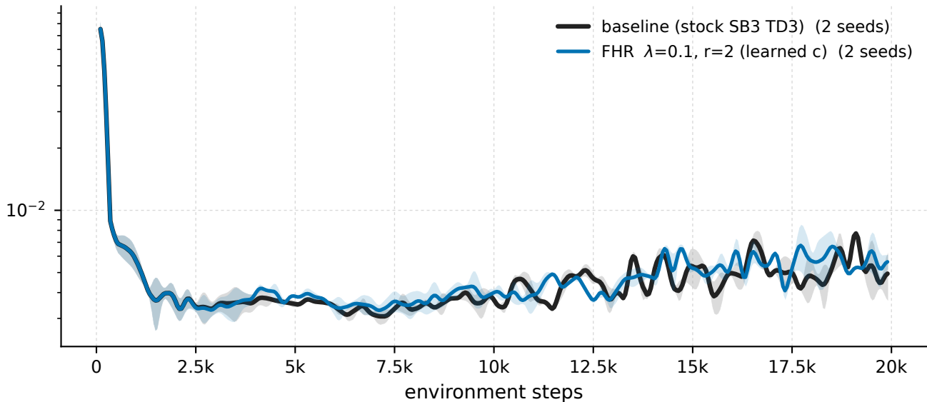
Pendulum-v1 - \lambda 0.1 \cdot r_2 vs baseline, penalised windows penalty-block tail \sigma_{r+1}/\sigma_1
