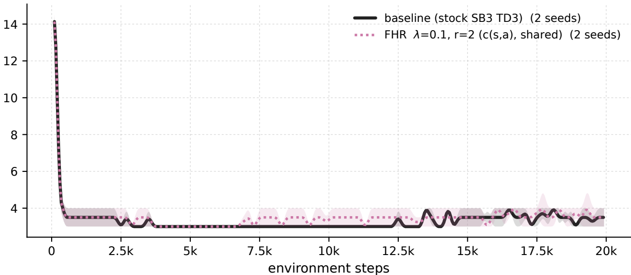
Pendulum-v1 - \lambda 0.1 \cdot r_2 c(s,a) shared vs baseline, penalised windows energy rank @ 99.9%
