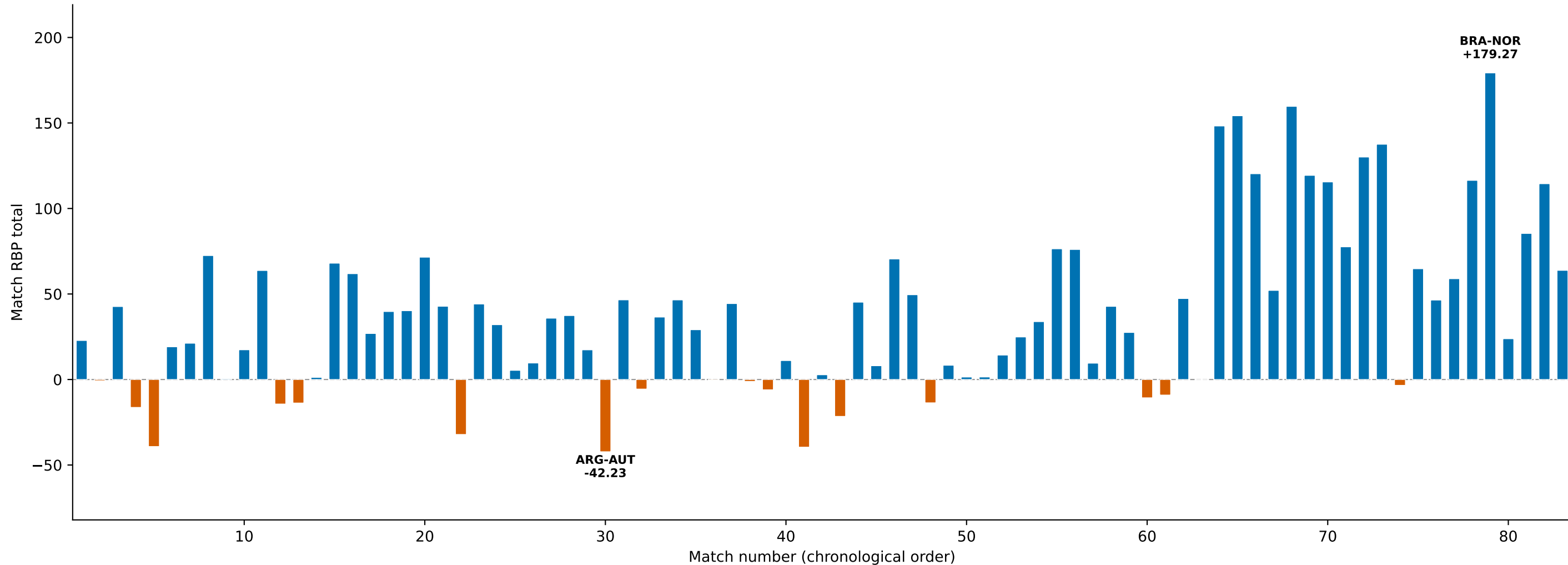
JTC Campaign Track Record: RBP by Match (sign-coded)
