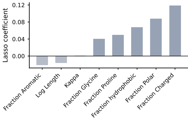
Reference distribution of lasso coefficients
