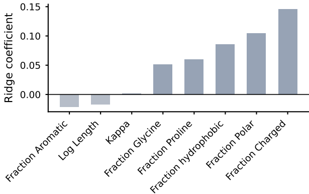
Reference distribution of ridge coefficients
