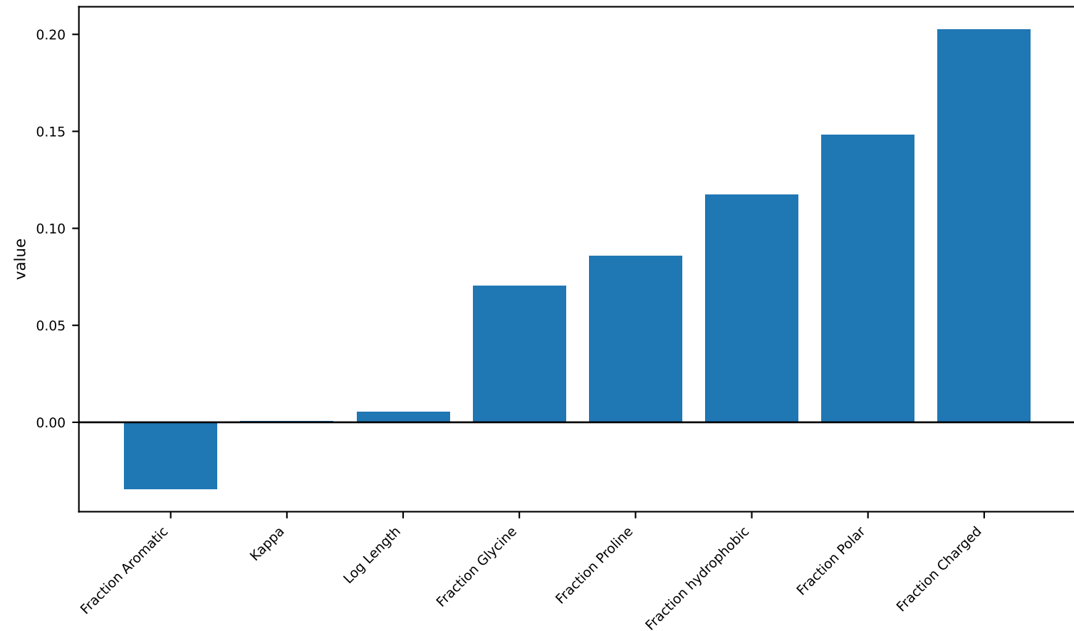
Lasso feature coefficients
